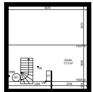
Zolder
